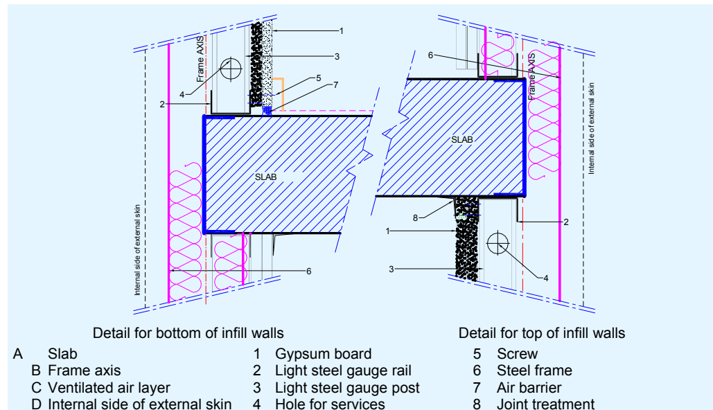
Figure 5.6 Infill walls
